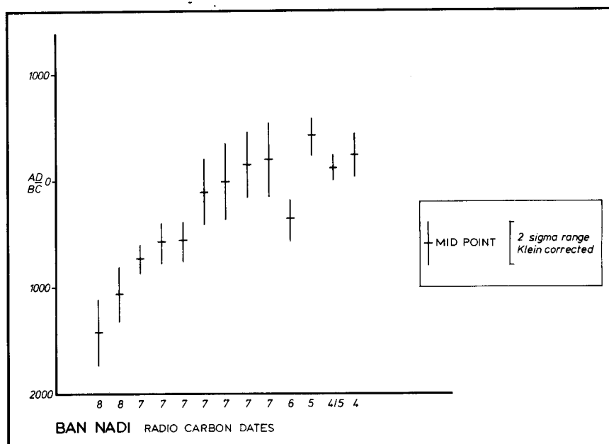
FIG. 3. The distribution of radio-carbon dates from Ban Nadi, set against their layer of origin.
